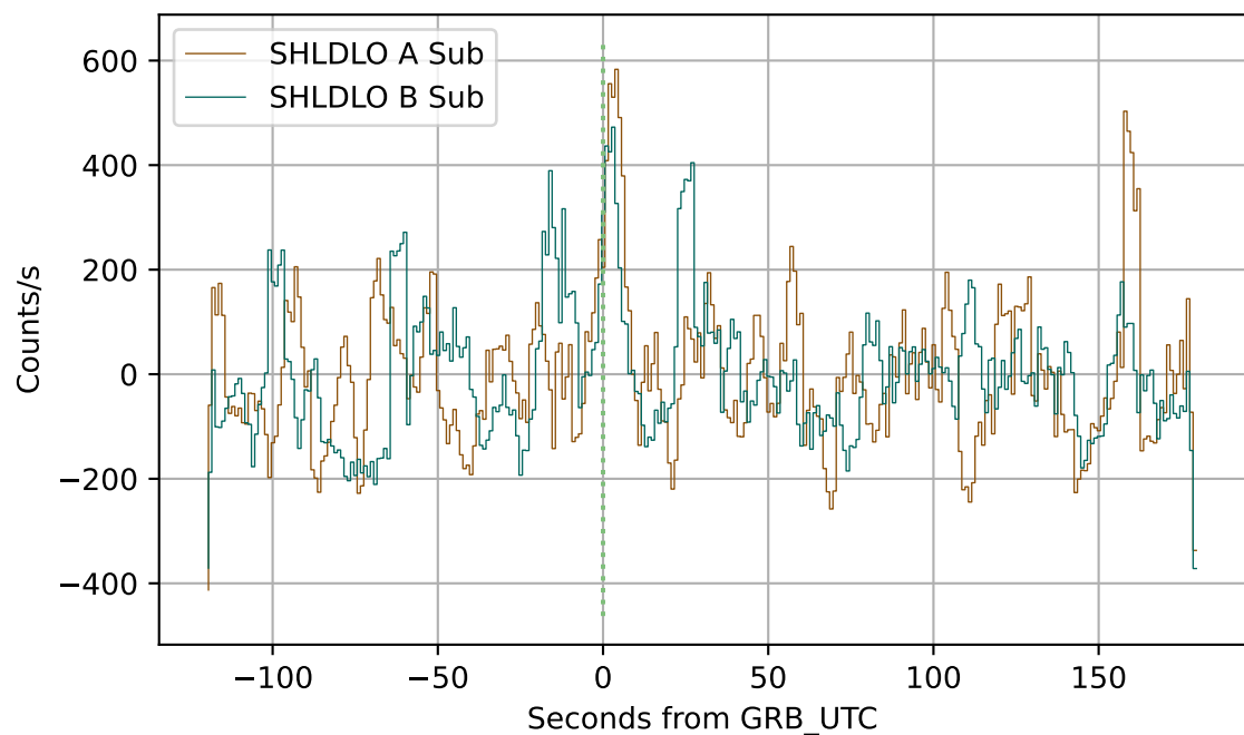
GOES X-ray Flux
