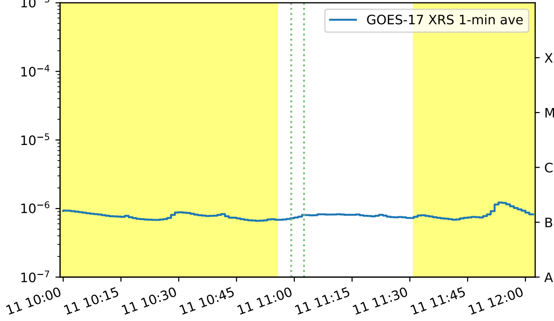
GOES X-ray Flux
