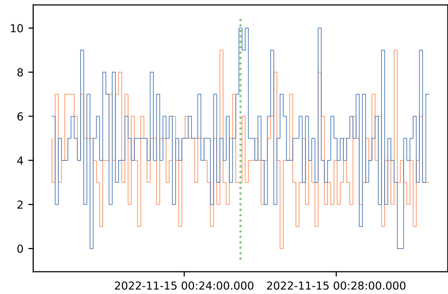
E > 100 keV, 0.25-s bins
