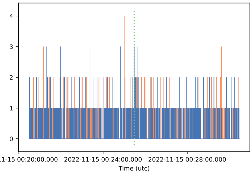
E > 100 keV, 0.25-s bins
