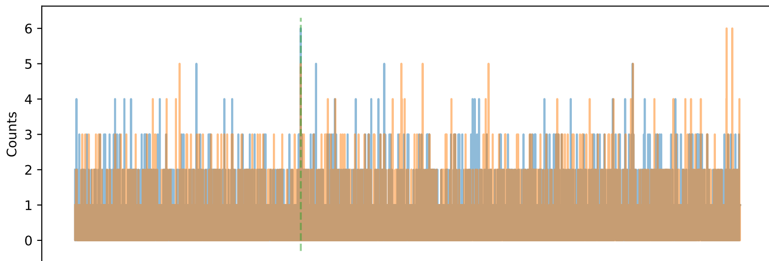
Counts in 0.25 bins
