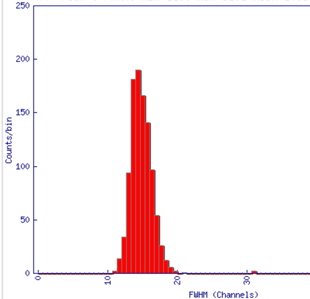
H44 Peak 0 FWHM: min=11.0 max=31.1 mean=14.8
