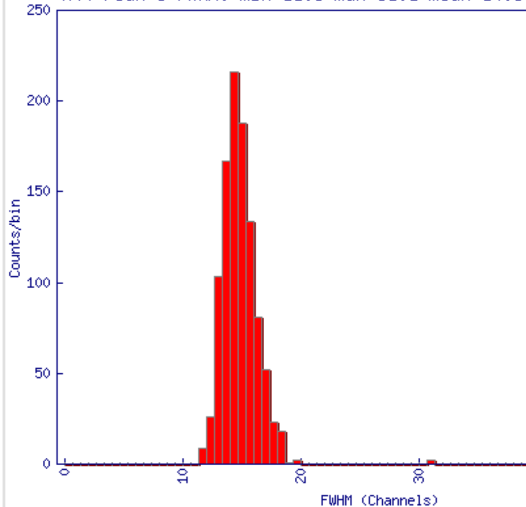
H44 Peak 3 FWHM: min=11.3 max=31.1 mean=14.8
