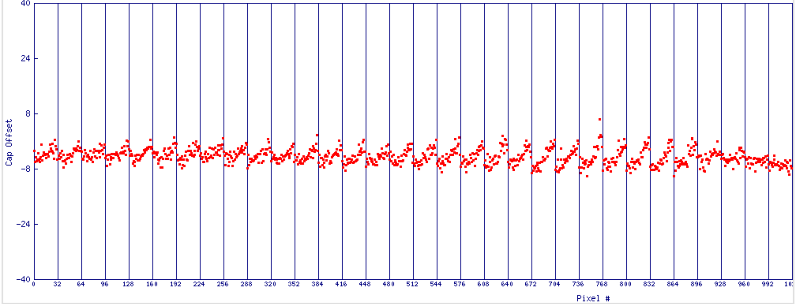
H44 Cap 10 Offset vs Pixel#
