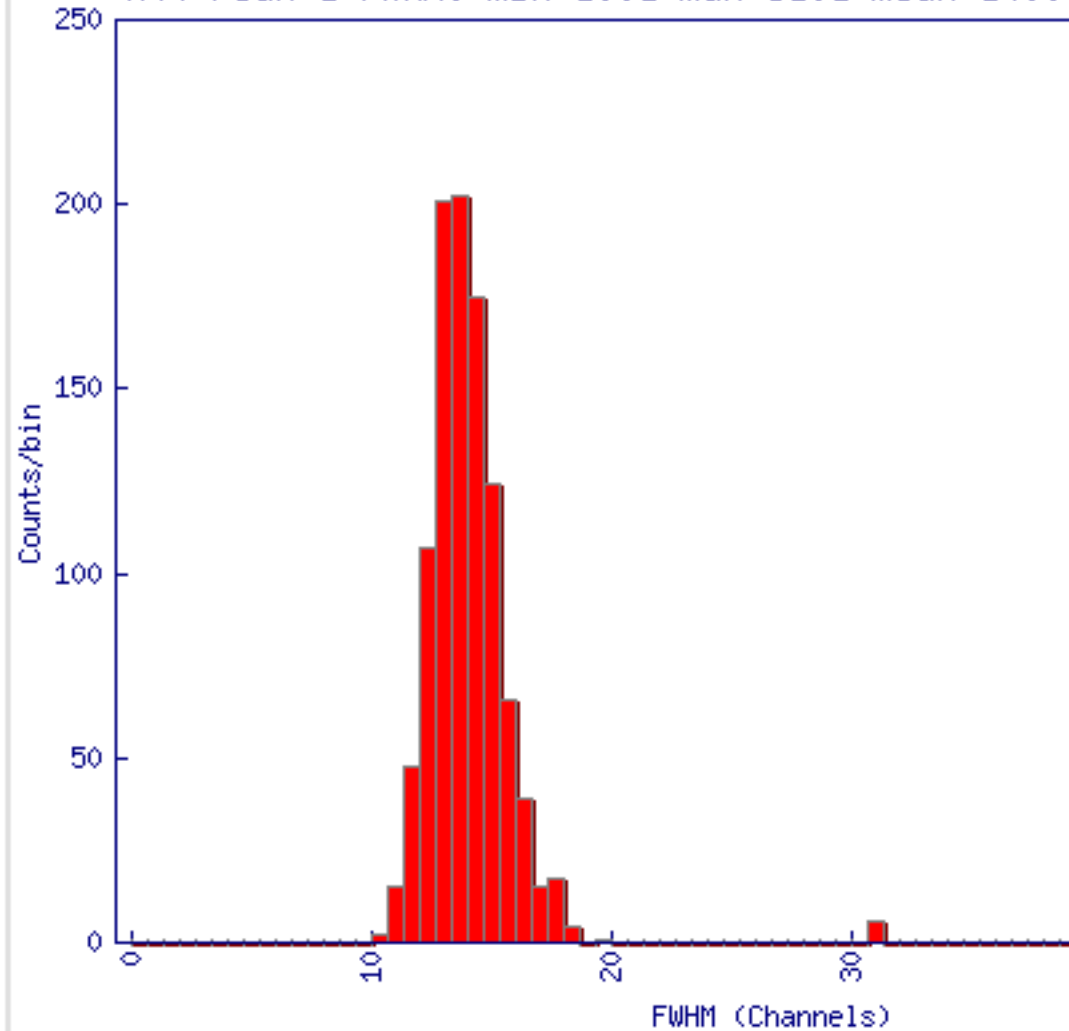
H44 Peak 1 FWHM: min=10.1 max=31.1 mean=14.0
