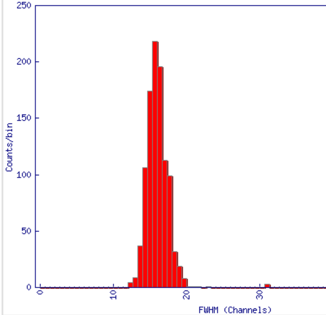
H44 Peak 4 FWHM: min=12.2 max=31.1 mean=16.0
