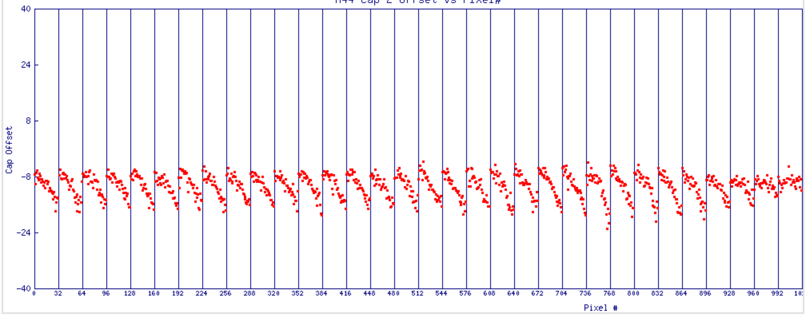
H44 Cap 2 Offset vs Pixel#
