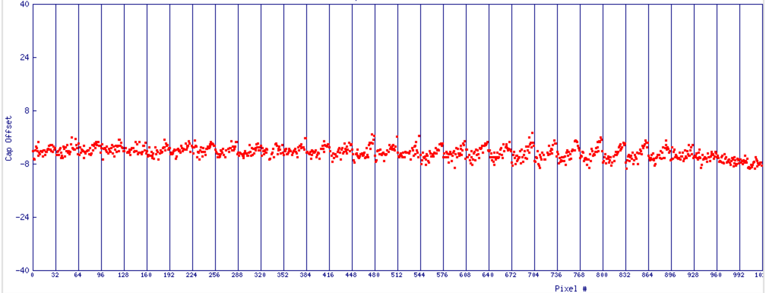
H43 Cap 5 Offset vs Pixel#
