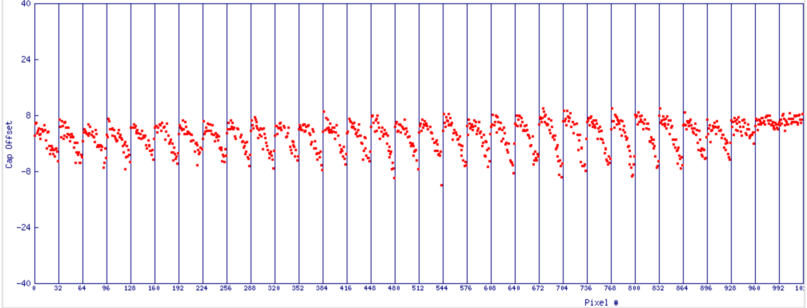
H43 Cap 15 Offset vs Pixel#
