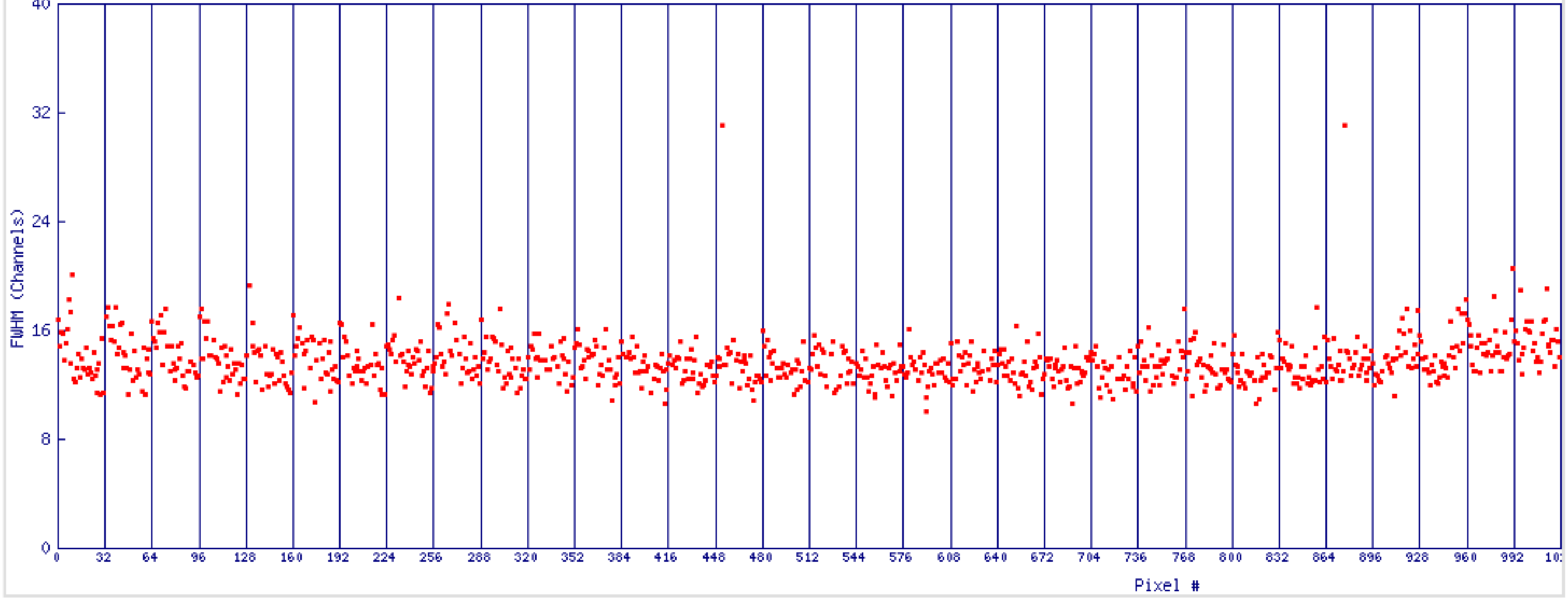
H43 Peak 1 FWHM vs Pixel#. min=10.1 max=31.1 mean=13.7
