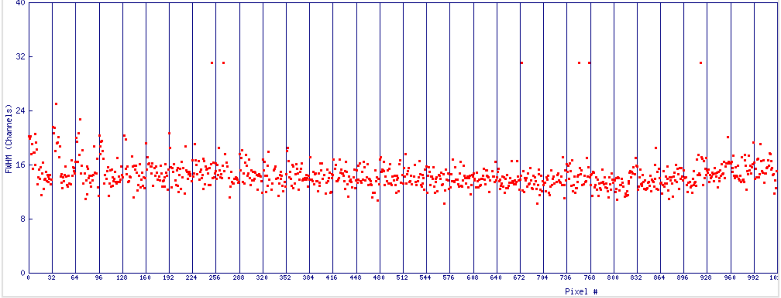
H43 Peak 0 FWHM vs Pixel#. min=10.3 max=31.1 mean=14.6
