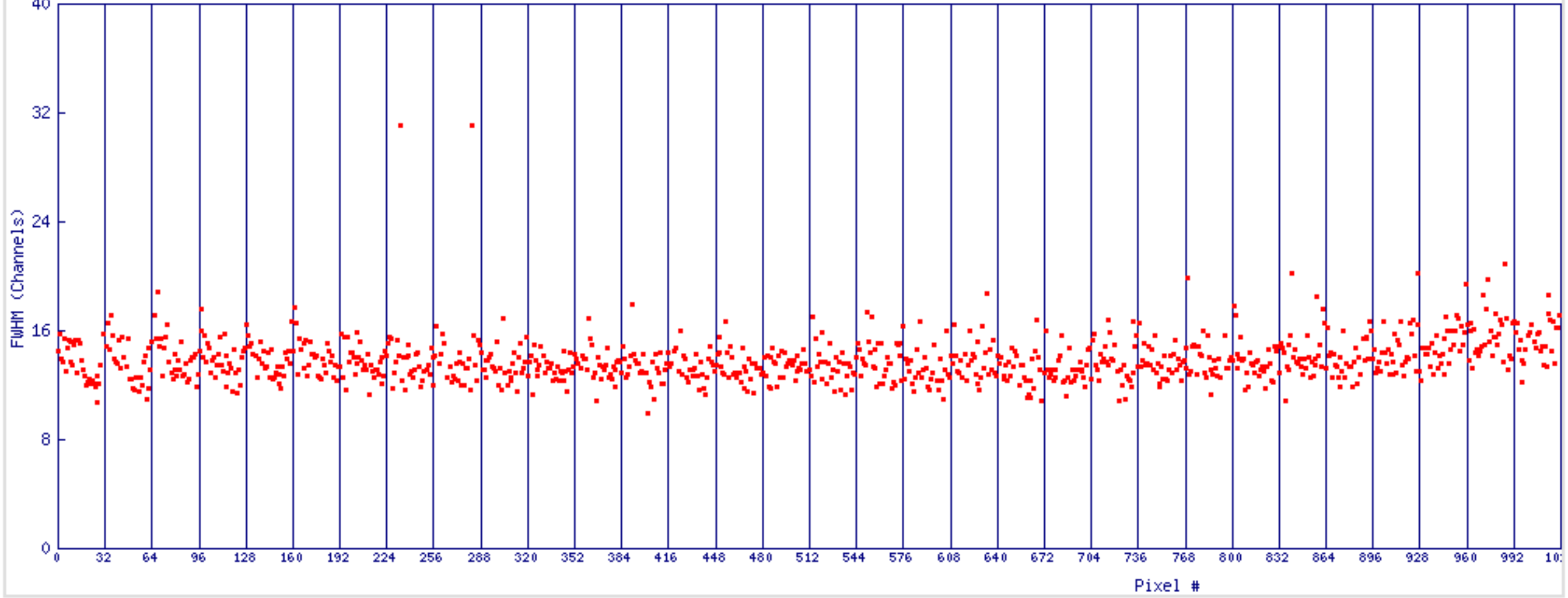
H36 Peak 1 FWHM vs Pixel#. min= 9.9 max=31.1 mean=13.9
