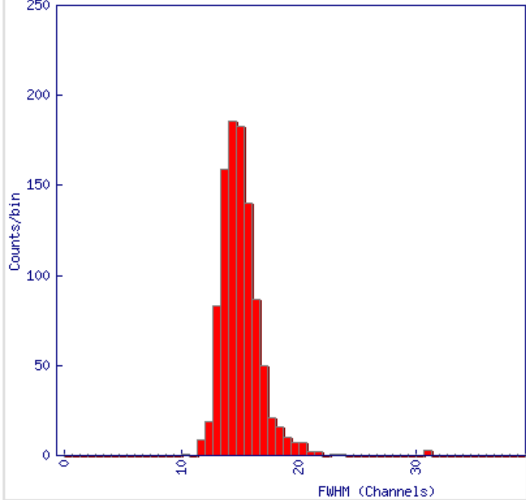
H36 Peak 3 FWHM: min=10.6 max=31.1 mean=15.0
