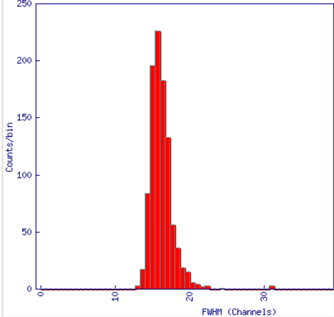
H36 Peak 4 FWHM: min=12.9 max=31.1 mean=16.2
