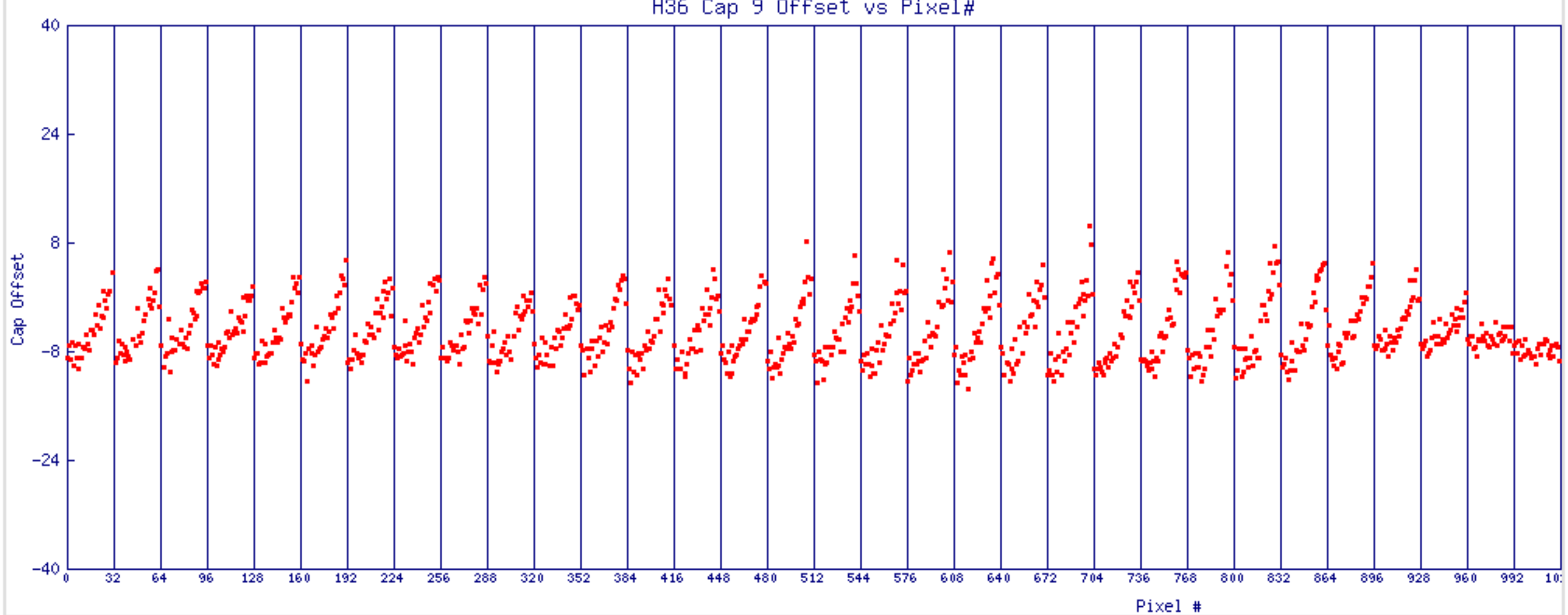
H36 Cap 9 Offset vs Pixel#
