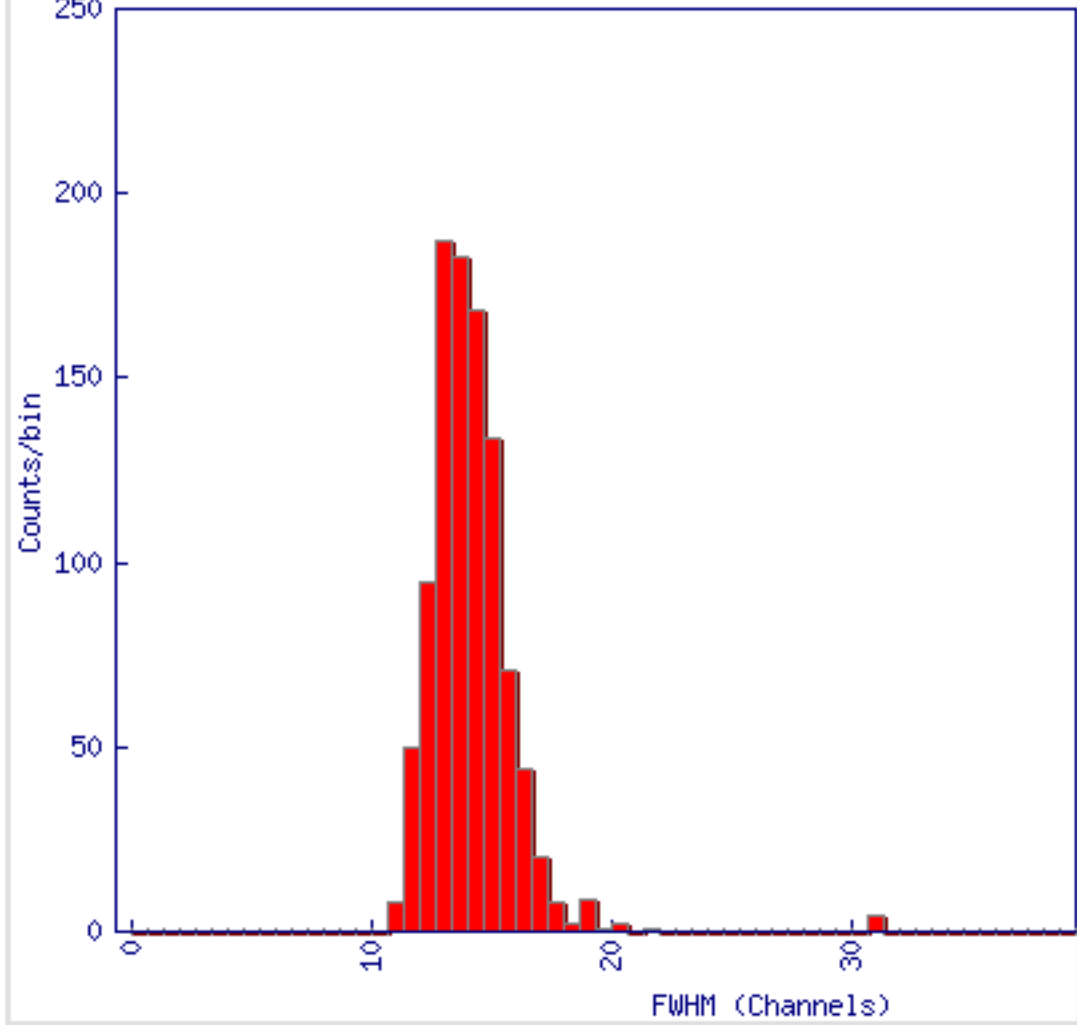
H36 Peak 0 FWHM: min=11.0 max=31.1 mean=14.1
