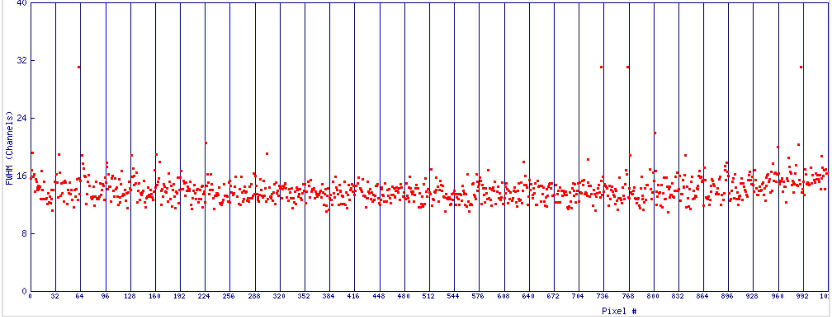
H36 Peak 0 FWHM vs Pixel#. min=11.0 max=31.1 mean=14.1
