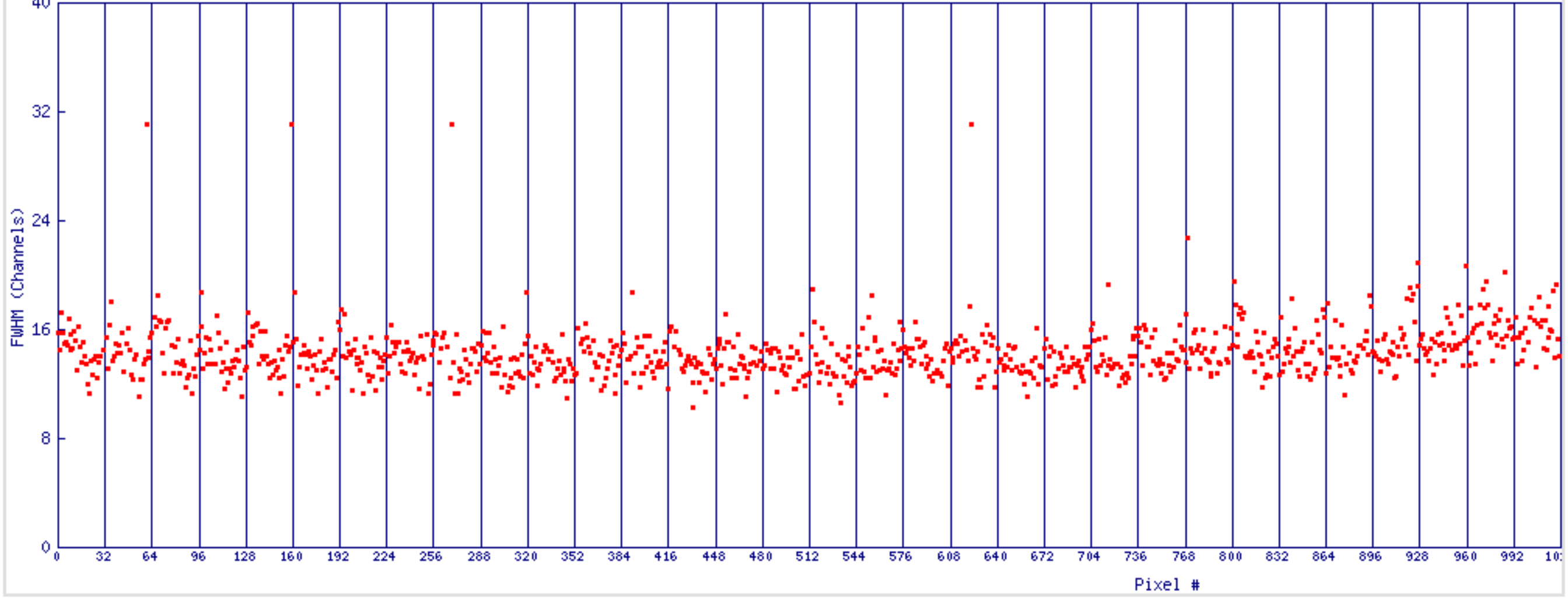
H36 Peak 2 FWHM vs Pixel#. min=10.3 max=31.1 mean=14.3
