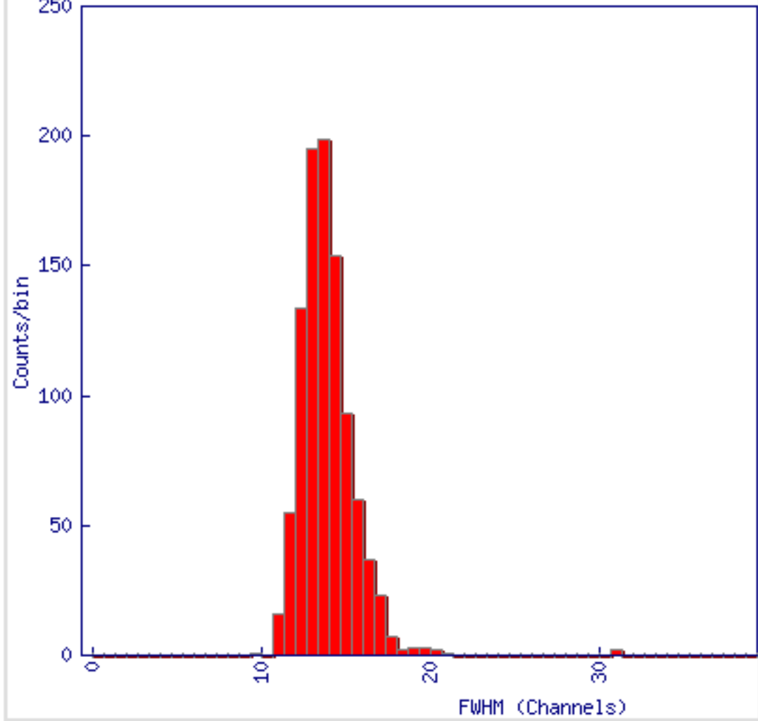
H36 Peak 1 FWHM: min= 9.9 max=31.1 mean=13.9
