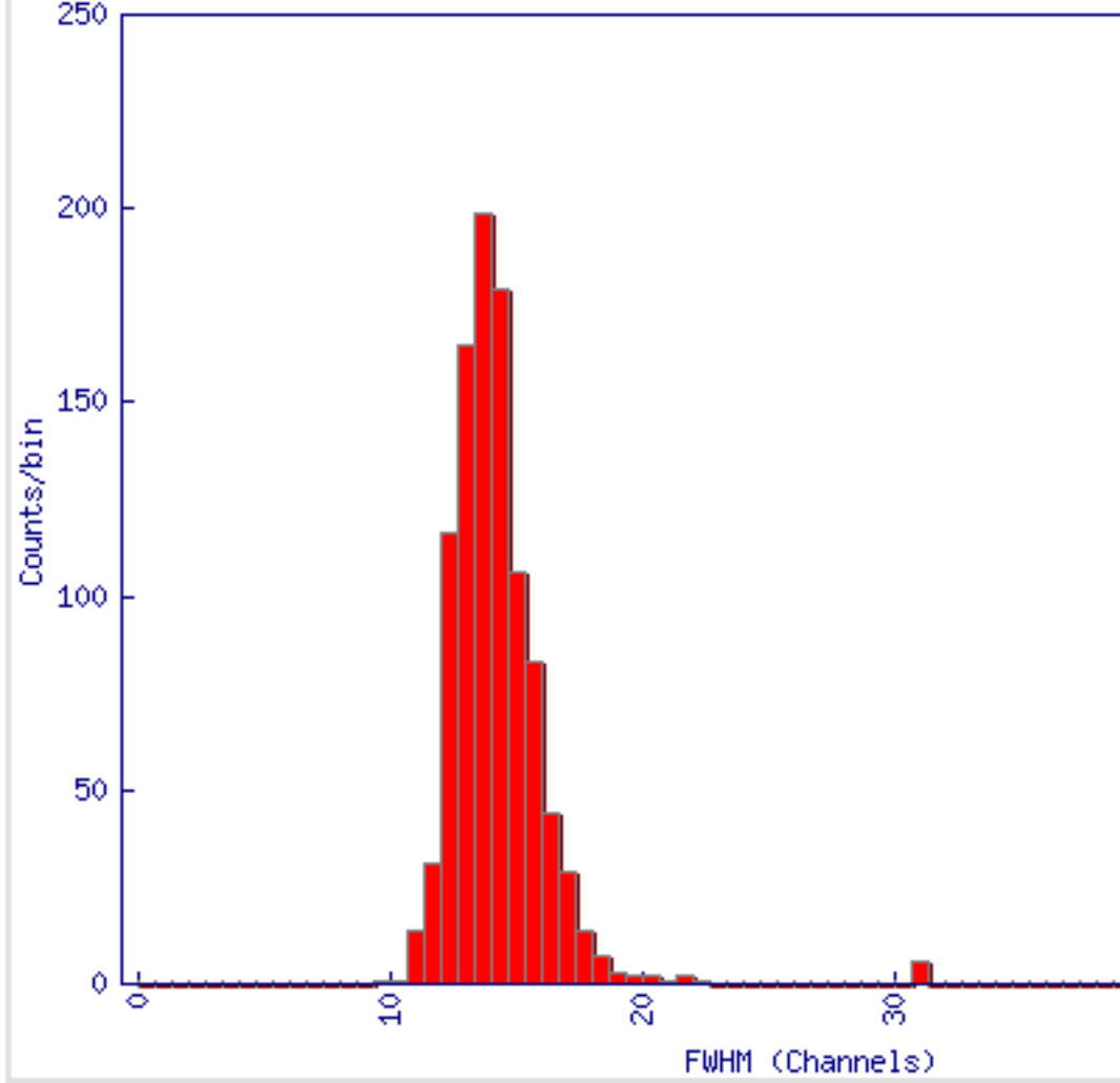
H35 Peak 2 FWHM: min= 9.8 max=31.1 mean=14.2
