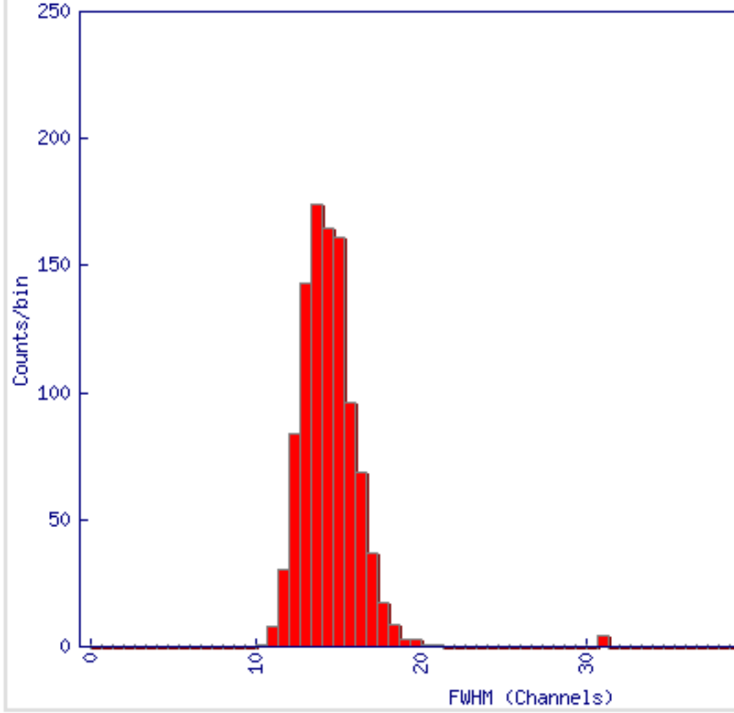
H35 Peak 0 FWHM: min=10.4 max=31.1 mean=14.4
