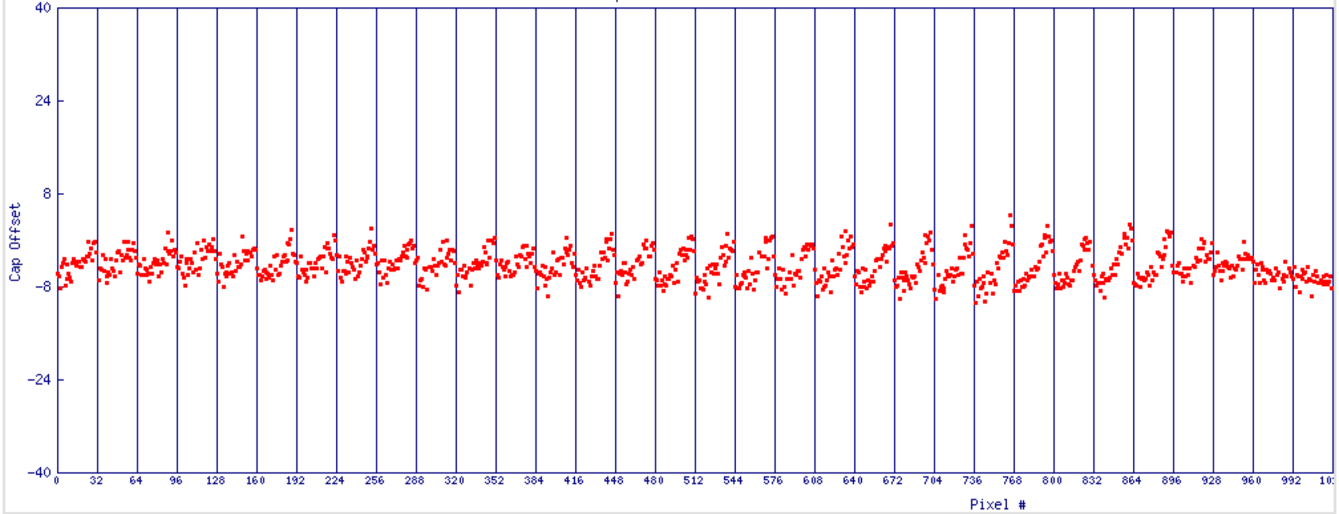
H35 Cap 10 Offset vs Pixel#
