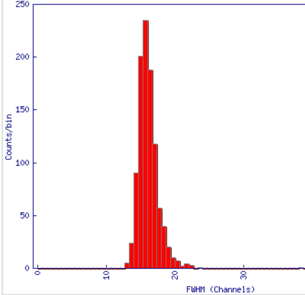
H35 Peak 4 FWHM: min=12.9 max=38.0 mean=16.1
