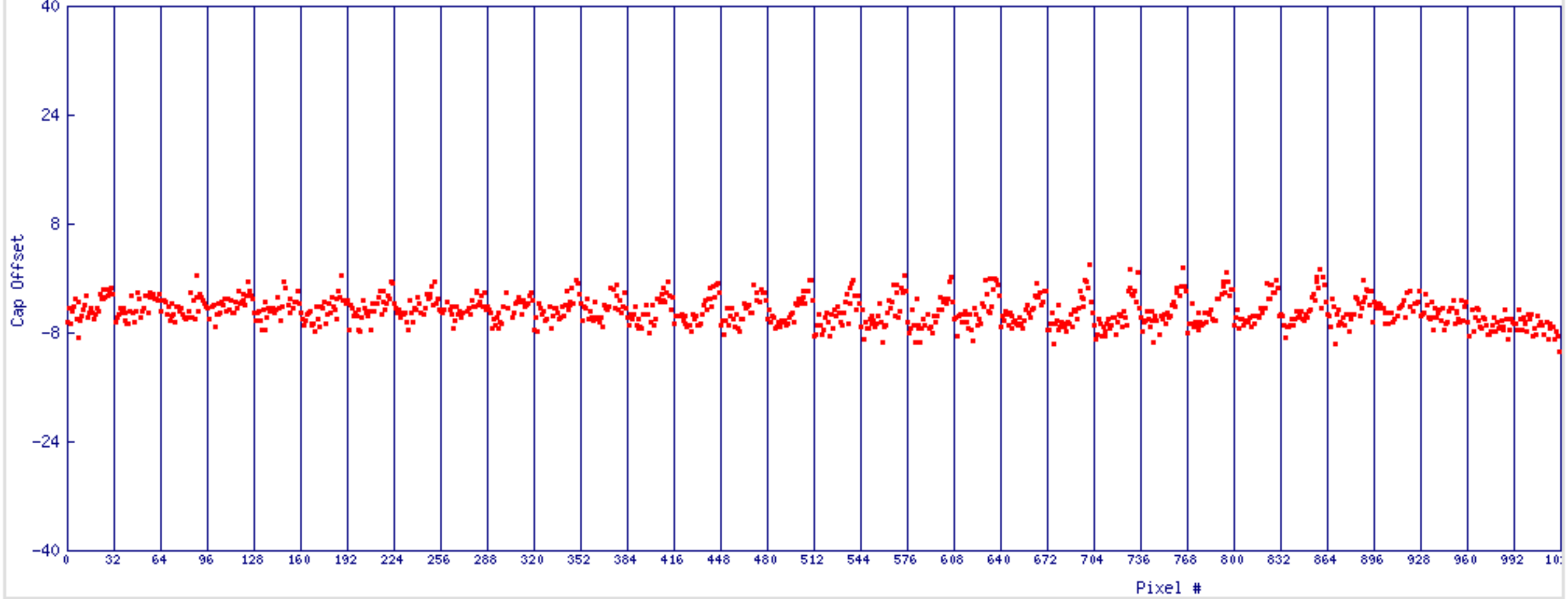
H35 Cap 5 Offset vs Pixel#
