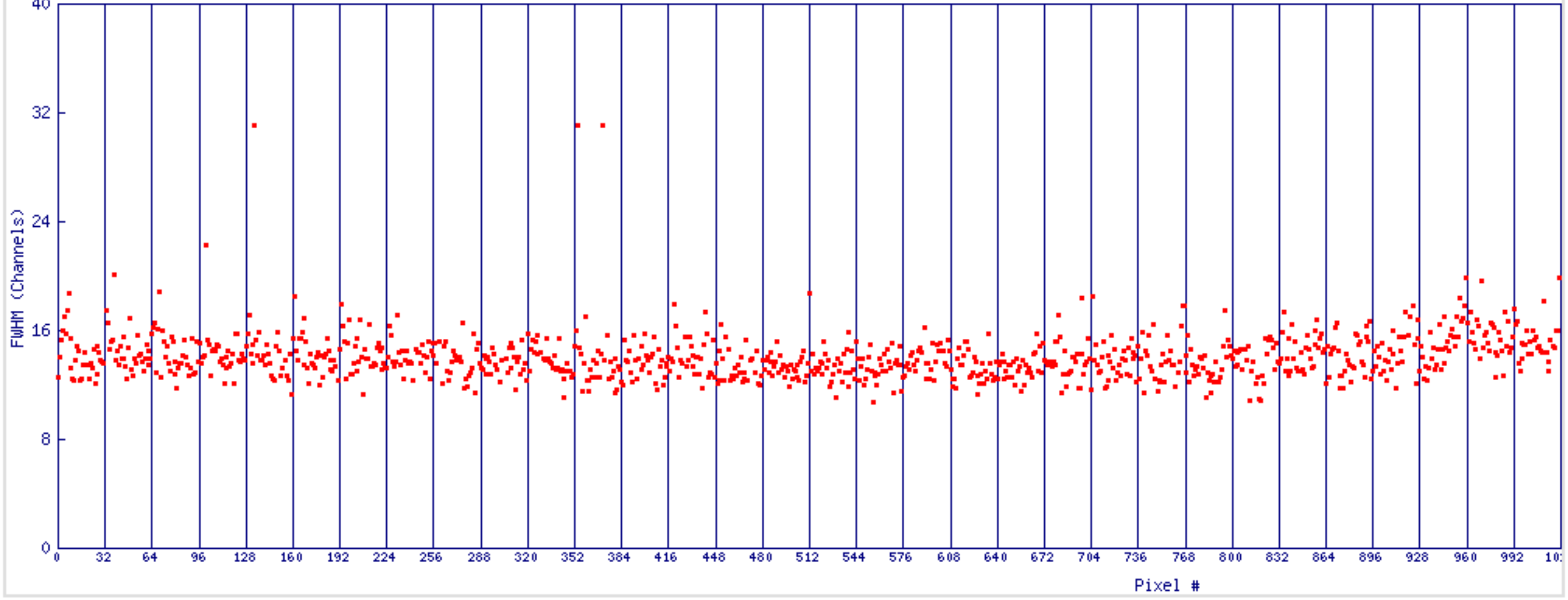
H35 Peak 1 FWHM vs Pixel#. min=10.7 max=31.1 mean=14.1
