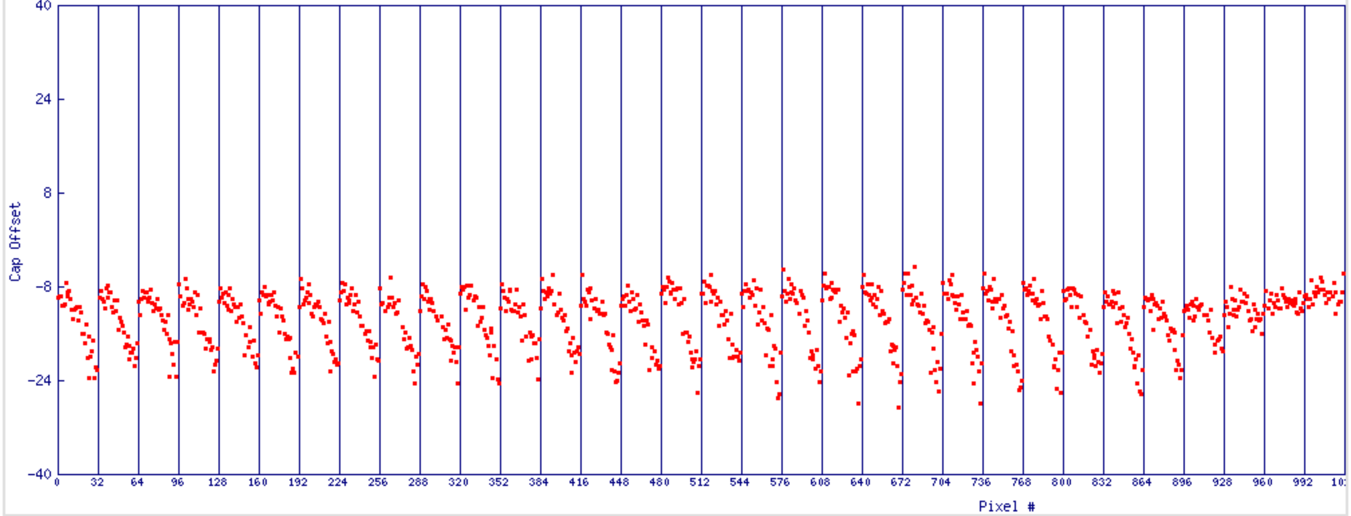
H35 Cap 14 Offset vs Pixel#
