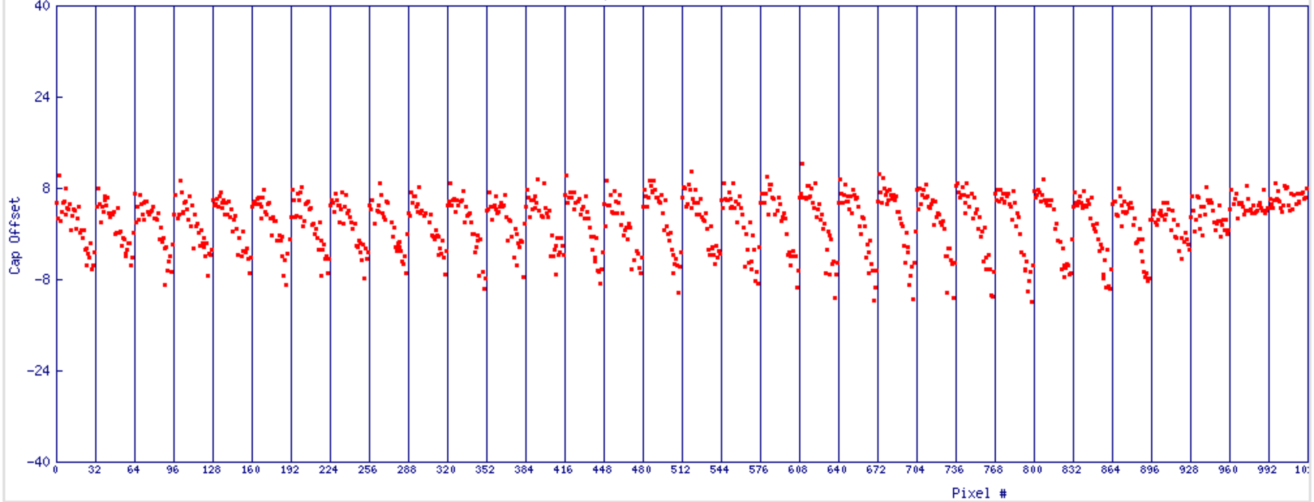
H35 Cap 15 Offset vs Pixel#
