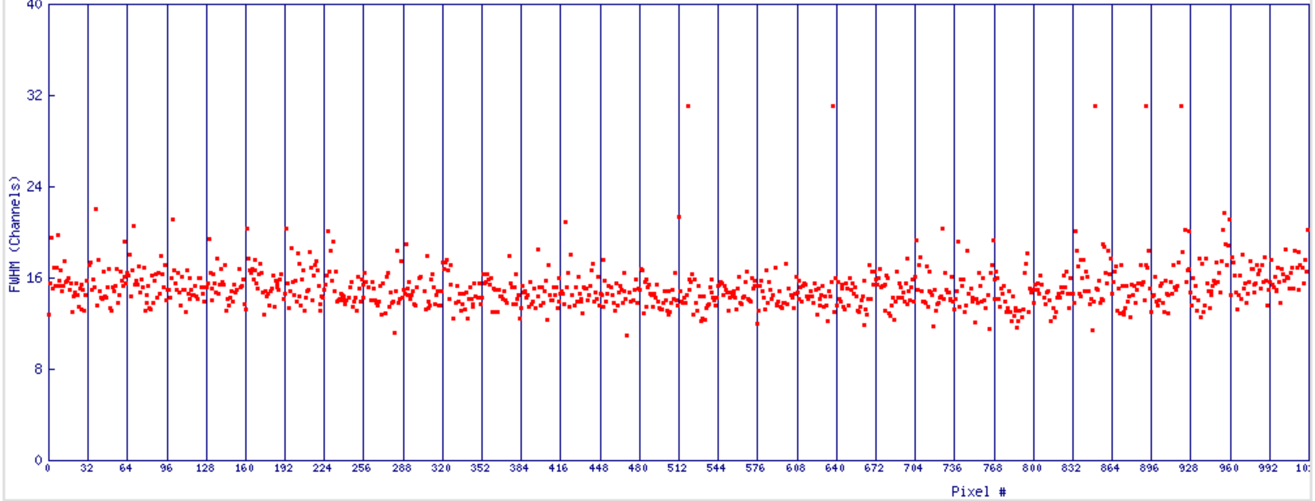
H35 Peak 3 FWHM vs Pixel#. min=10.9 max=31.1 mean=15.2
