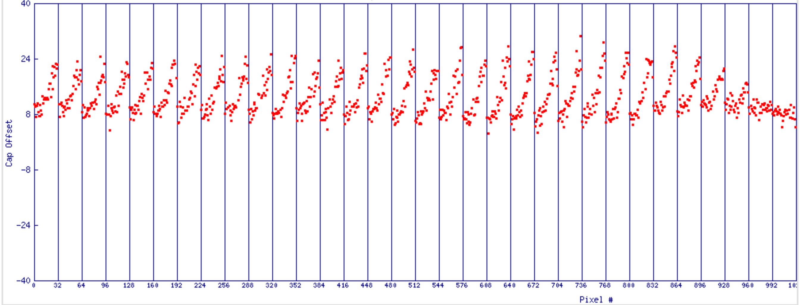
H35 Cap 7 Offset vs Pixel#
