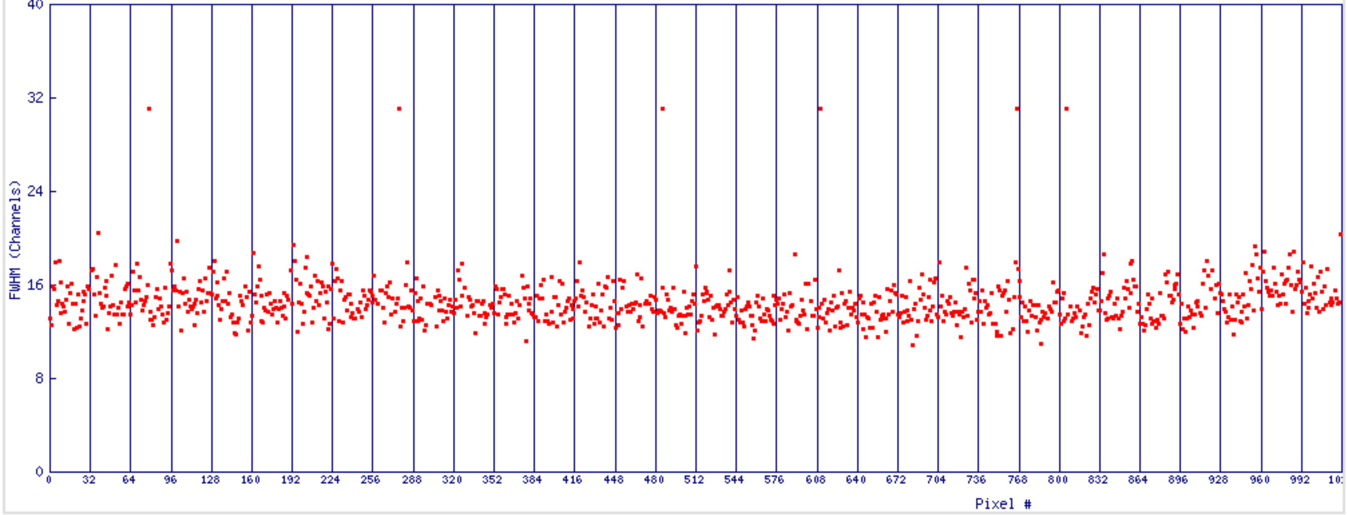
H35 Peak 0 FWHM vs Pixel#. min=10.8 max=31.1 mean=14.6
