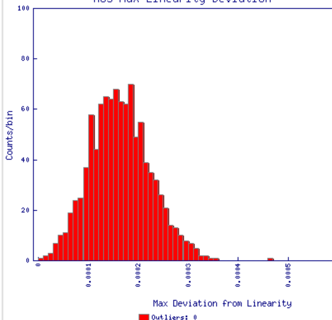
H35 Max Linearity Deviation
