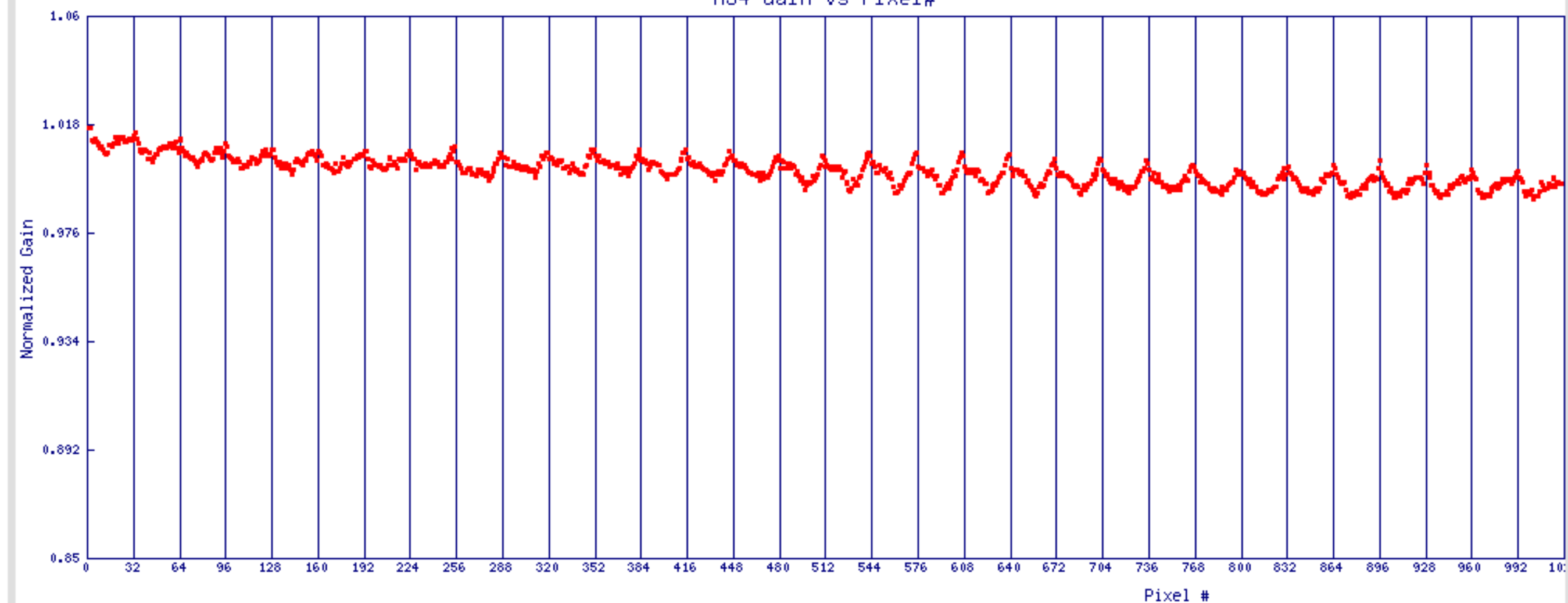
H34 Gain vs Pixel#
