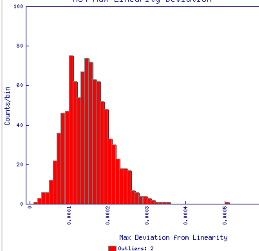
H34 Max Linearity Deviation
