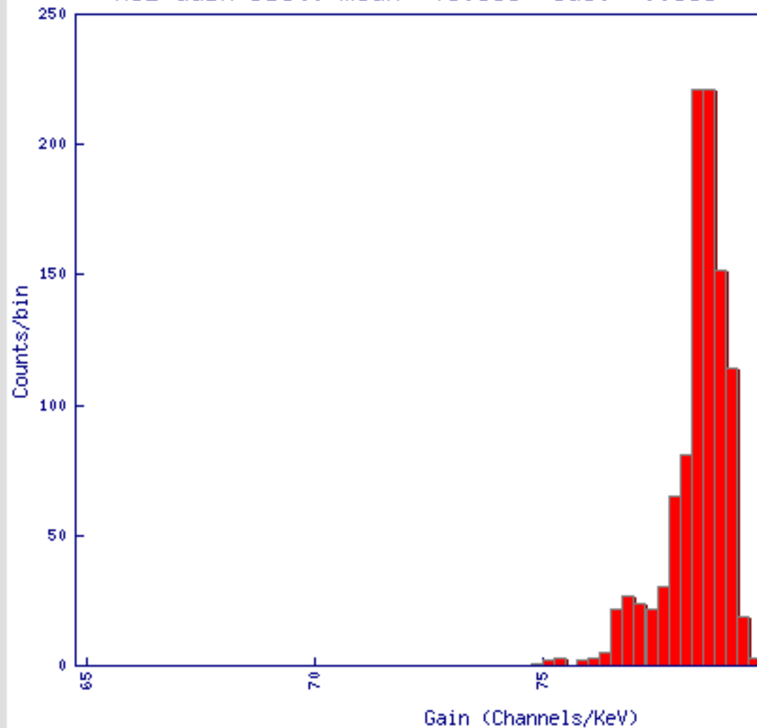
H32 Gain Dist: mean= 78.366 sdev= 0.683
