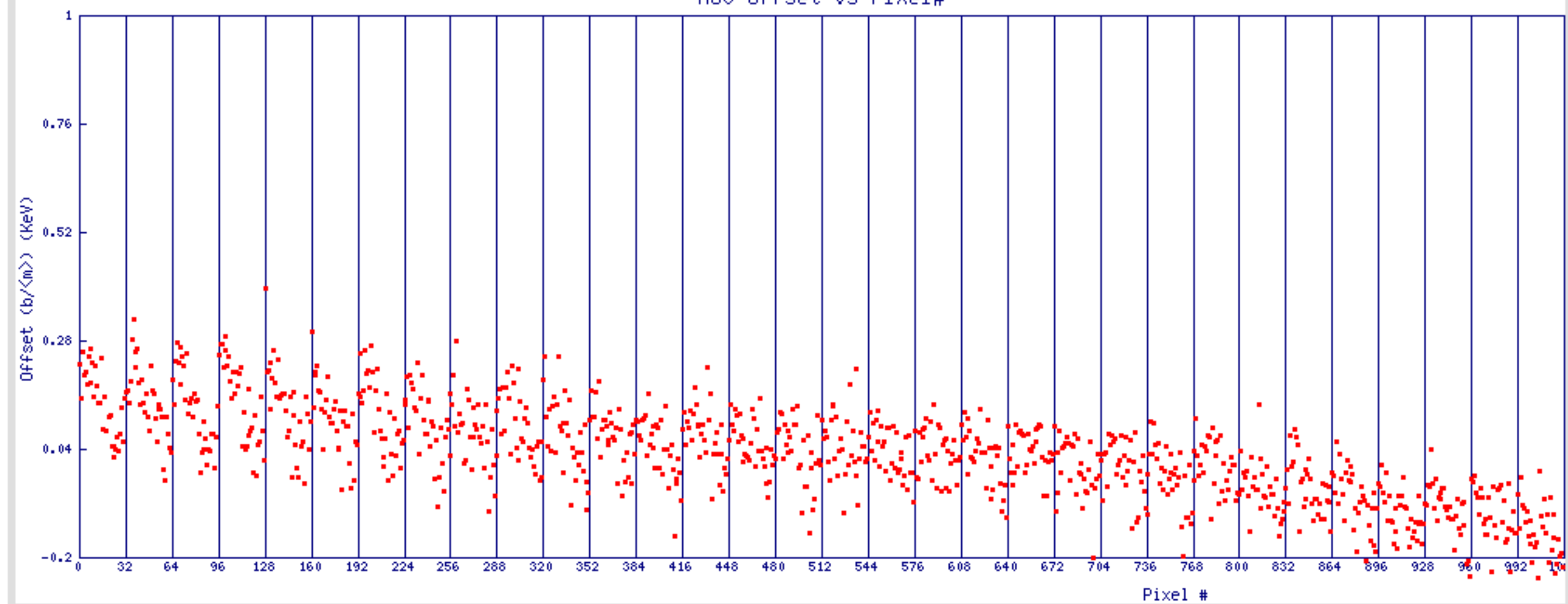
H30 Offset vs Pixel#
