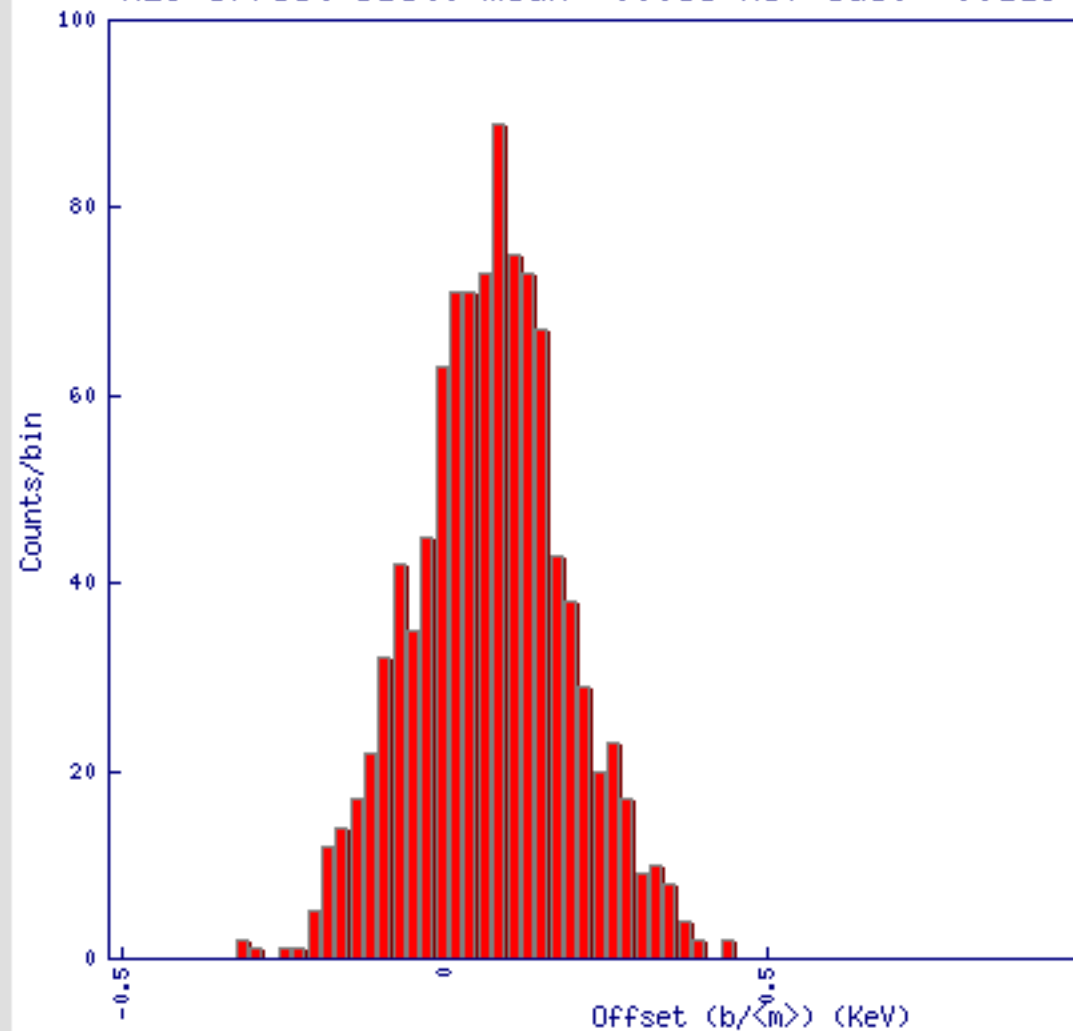
H29 Offset Dist: mean= 0.068 KeV sdev= 0.119
