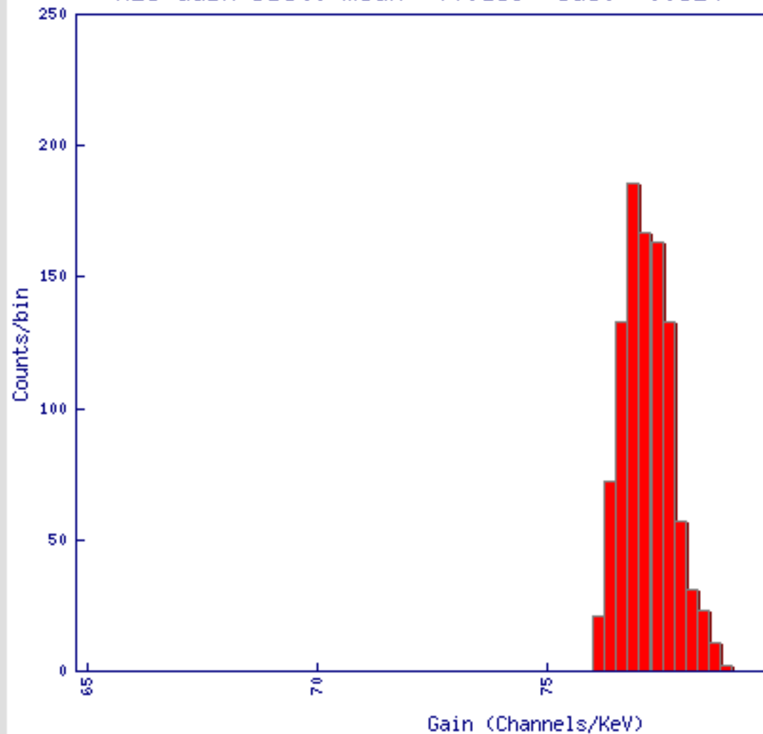
H28 Gain Dist: mean= 77.169 sdev= 0.524
