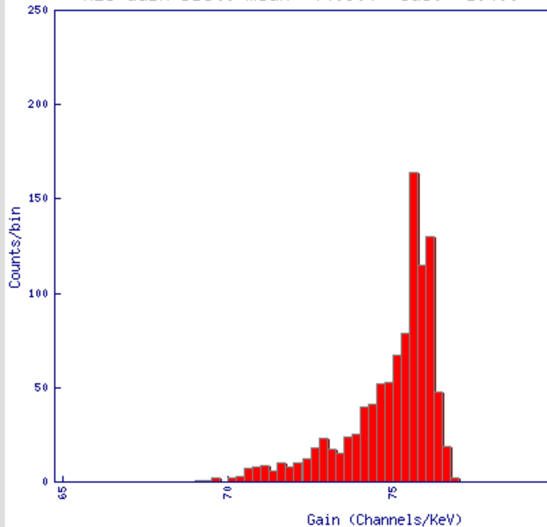
H25 Gain Dist: mean= 74.907 sdev= 1.400
