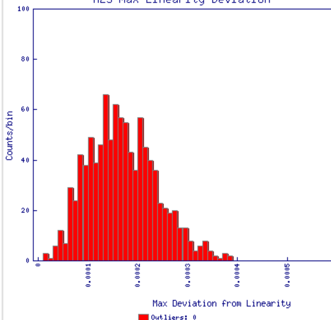
H25 Max Linearity Deviation
