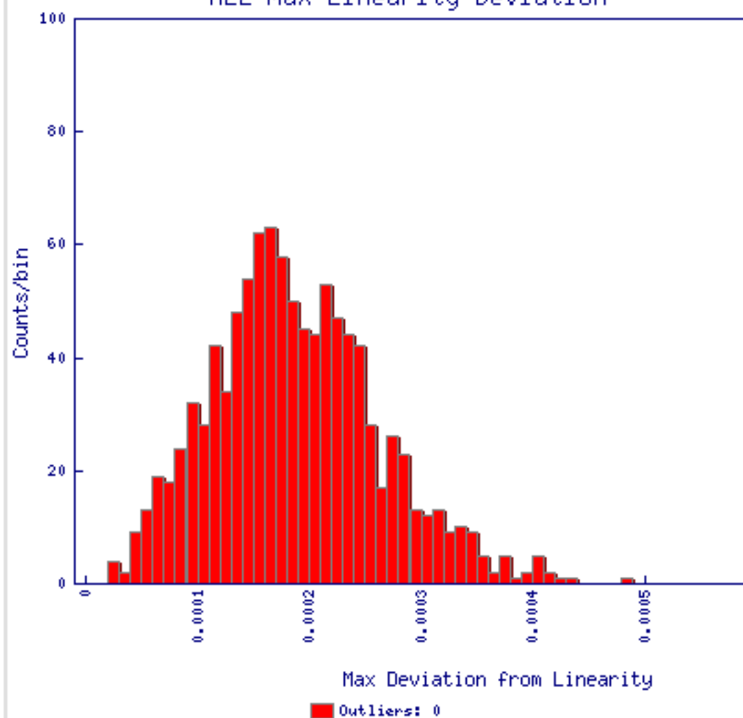
H22 Max Linearity Deviation
