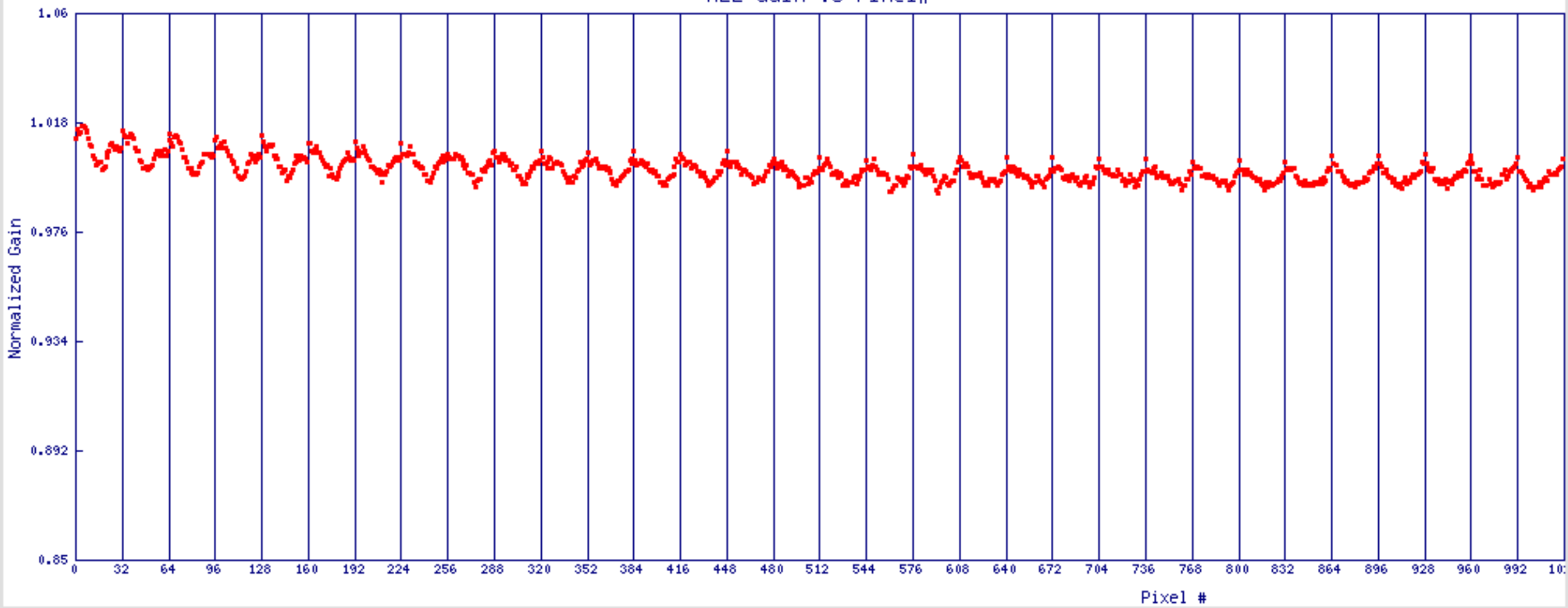
H22 Gain vs Pixel#
