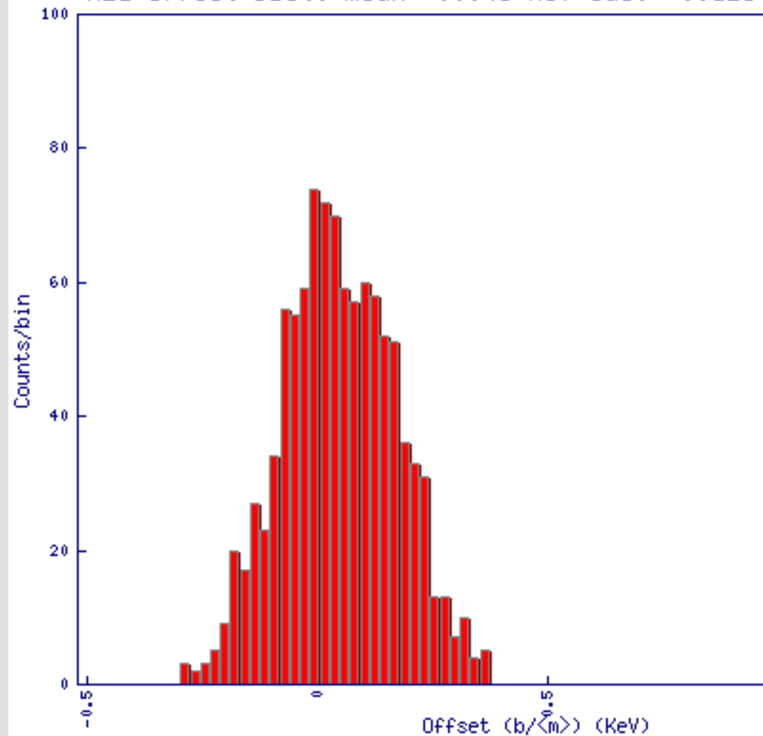
H21 Offset Dist: mean= 0.045 KeV sdev= 0.123
