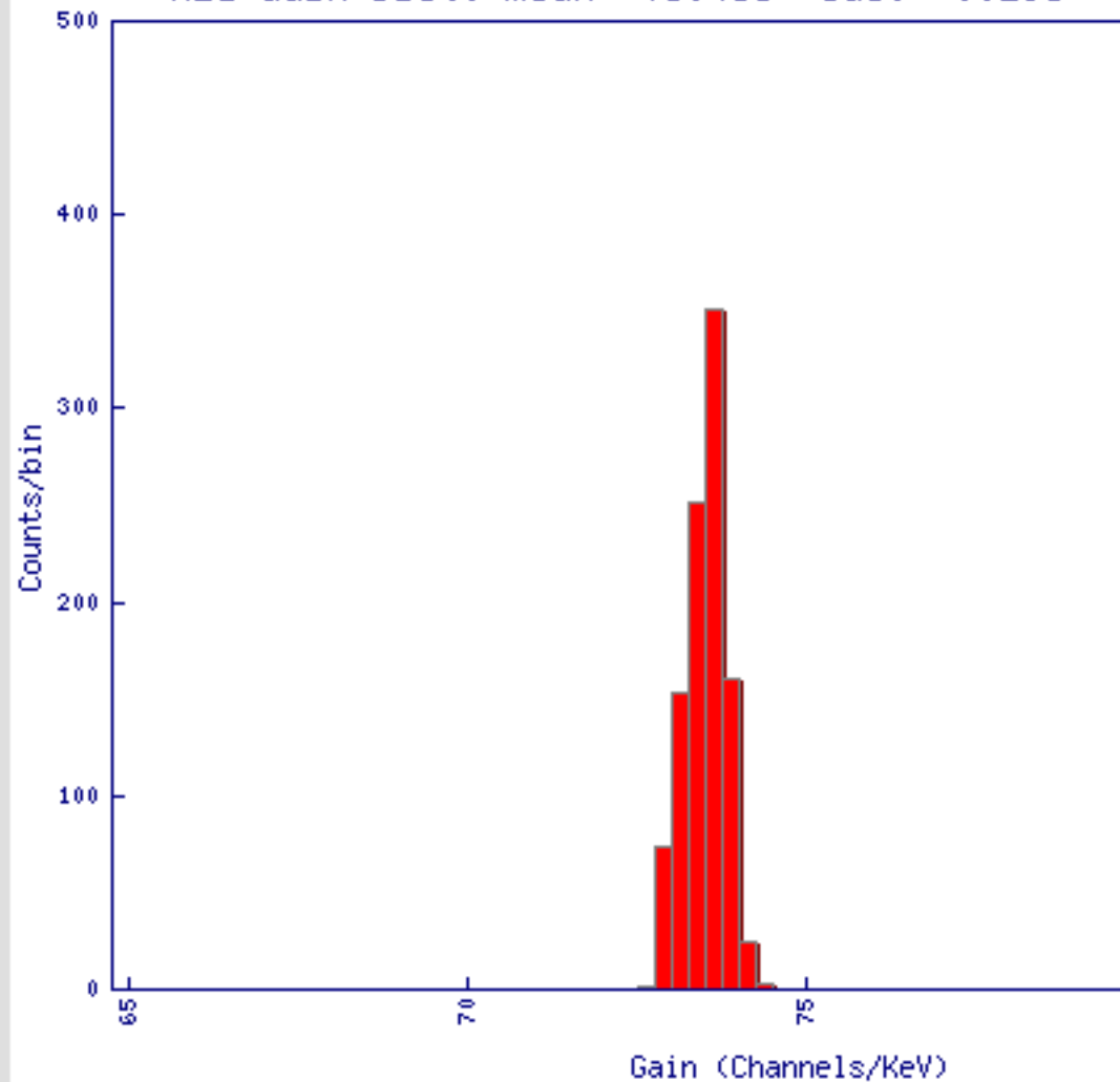
H21 Gain Dist: mean= 73.485 sdev= 0.296
