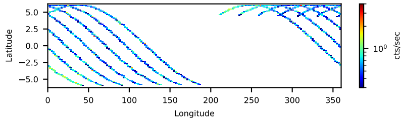
91002609004 FPMB: No SAA Filter 21.25-ks, 100%
