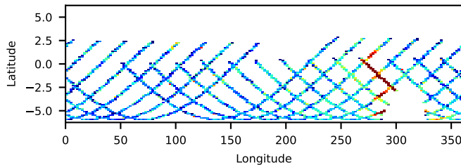
91002520002 FPMB: No SAA Filter 36.70-ks, 100%
