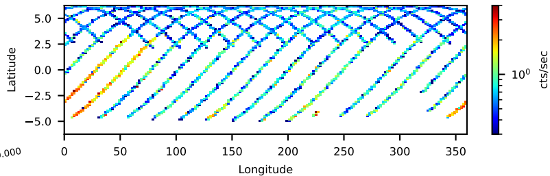
91001622002 FPMB: No SAA Filter 42.20-ks, 100%
