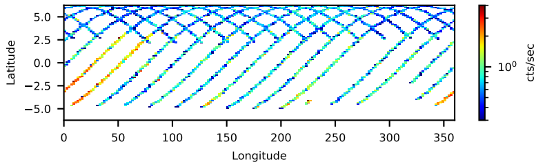
91001622002 FPMB: No SAA Filter 42.20-ks, 100%
