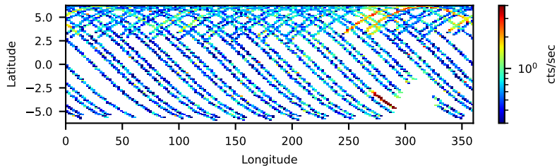
91001327002 FPMB: No SAA Filter 87.90-ks, 100%
