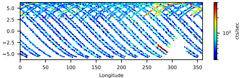
91001327002 FPMB: No SAA Filter 87.90-ks, 100%
