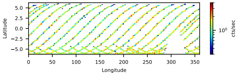
90901331002 FPMA: No SAA Filter 42.70-ks, 100%
