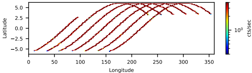
90801637002 FPMA: No SAA Filter 19.72-ks, 100%
