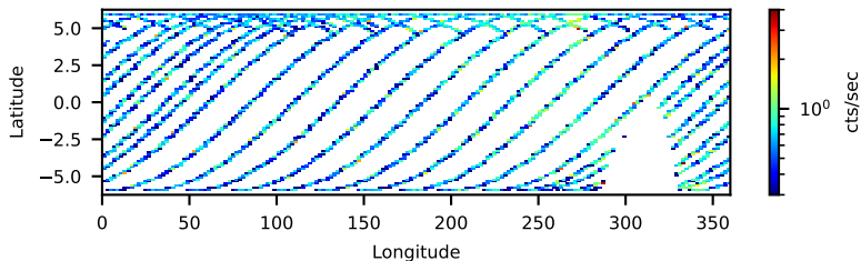
80902505002 FPMB: No SAA Filter 55.57-ks, 100%
