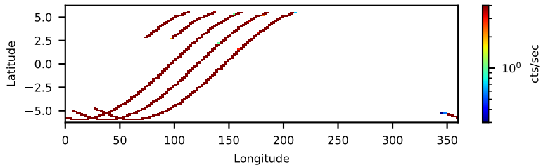
80902348001 FPMA: No SAA Filter 4.10-ks, 100%
