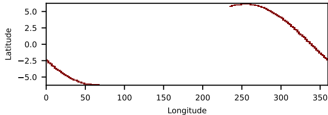
80902012004 FPMB: No SAA Filter 2.70-ks, 100%
