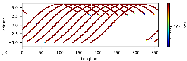
80802346002 FPMA: No SAA Filter 17.18-ks, 100%
