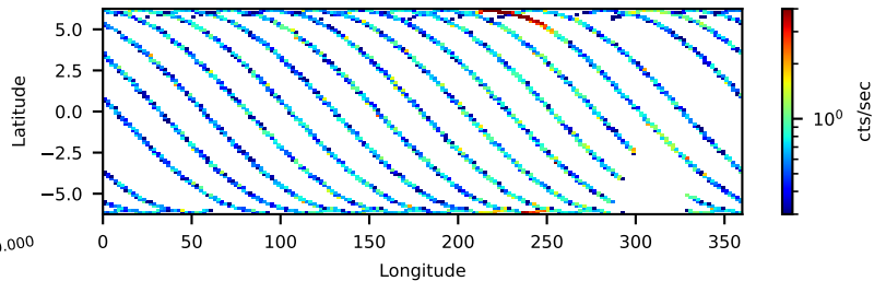
61002008004 FPMA: No SAA Filter 40.91-ks, 100%
