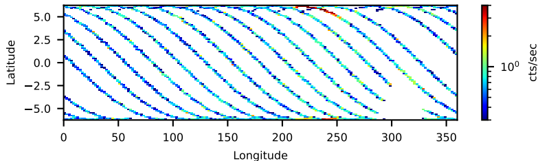
61002008004 FPMA: No SAA Filter 40.91-ks, 100%
