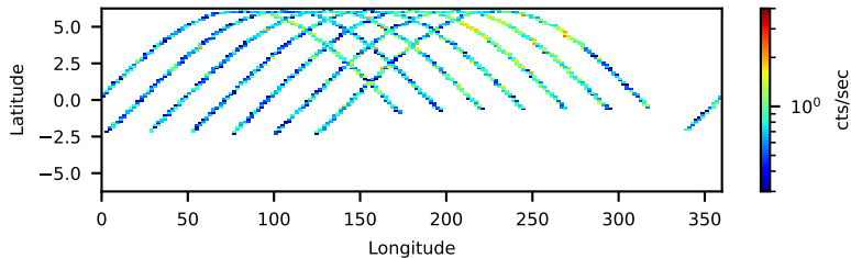
60964004002 FPMA: No SAA Filter 21.69-ks, 100%
