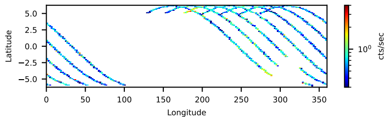
60963009002 FPMA: No SAA Filter 19.63-ks, 100%
