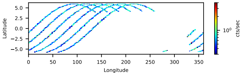
60963005002 FPMB: No SAA Filter 18.72-ks, 100%
