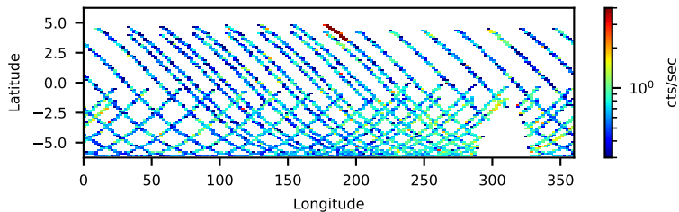
60910012002 FPMB: No SAA Filter 66.29-ks, 100%
