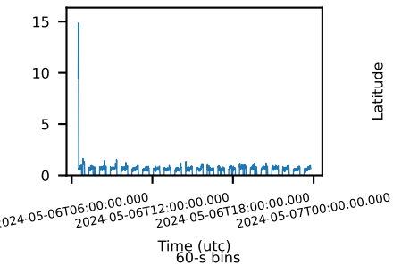
--saacalc=3 -saamode=OPTIMIZED --tentacle=yes 66.29-ks, 100%
