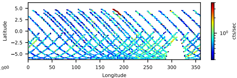
--saacalc=3 -saamode=OPTIMIZED --tentacle=yes 66.29-ks, 100%
