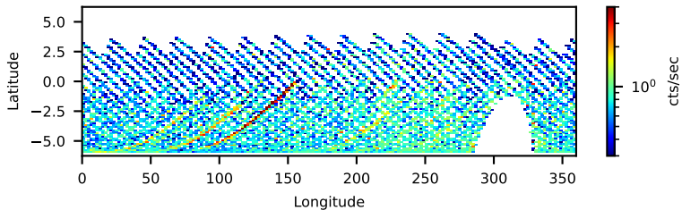
60902004002 FPMB: No SAA Filter 129.37-ks, 100%
