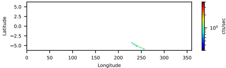
60864005001 FPMA: No SAA Filter 0.46-ks, 100%
