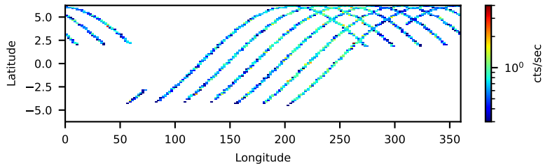
60864001002 FPMB: No SAA Filter 20.07-ks, 100%
