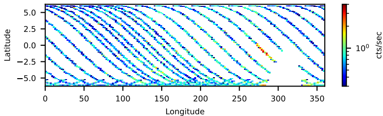
60863008002 FPMB: No SAA Filter 56.78-ks, 100%
