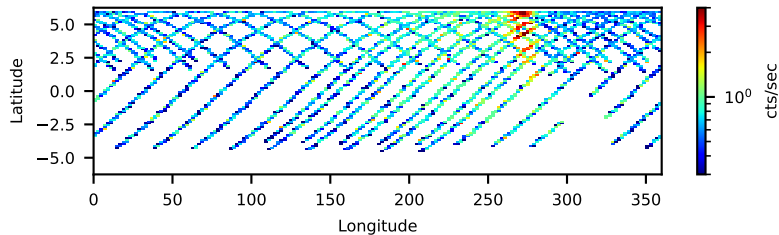
60862012002 FPMB: No SAA Filter 62.62-ks, 100%
