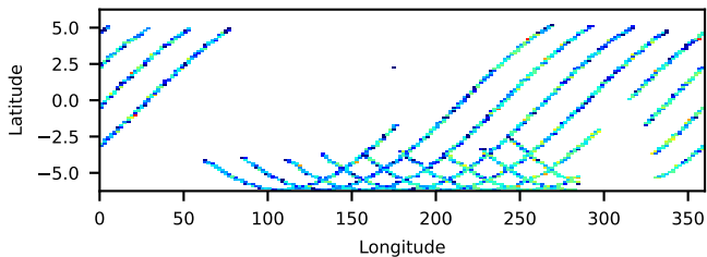
60860004002 FPMA: No SAA Filter 22.33-ks, 100%
