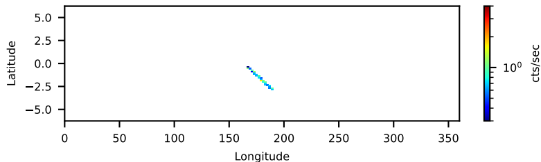
60802038007 FPMA: No SAA Filter 0.37-ks, 100%
