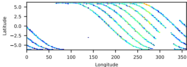
60802038006 FPMB: No SAA Filter 20.45-ks, 100%
