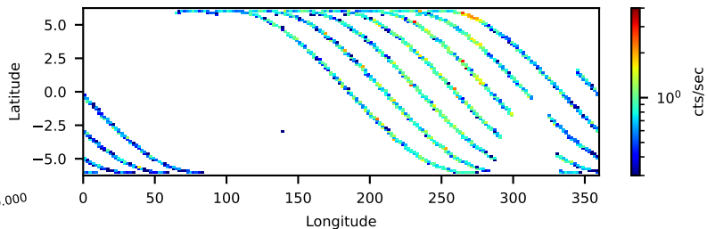
60802038006 FPMB: No SAA Filter 20.45-ks, 100%
