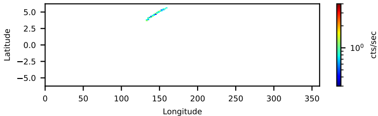
60802036003 FPMB: No SAA Filter 0.44-ks, 100%
