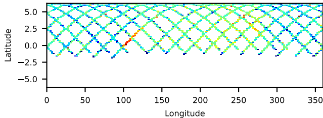
60802036002 FPMA: No SAA Filter 43.67-ks, 100%
