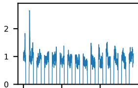
60-s bins
