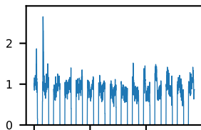
60-s bins
