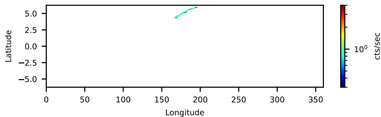
60802036001 FPMA: No SAA Filter 0.46-ks, 100%
