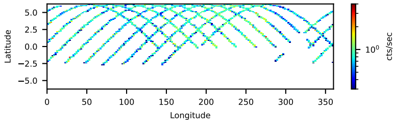
60667007002 FPMB: No SAA Filter 30.47-ks, 100%
