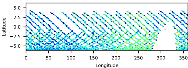
60601034002 FPMB: No SAA Filter 73.36-ks, 100%
