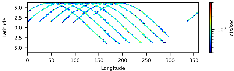
60464131002 FPMB: No SAA Filter 20.66-ks, 100%
