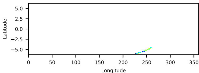
60464083001 FPMB: No SAA Filter 0.49-ks, 100%
